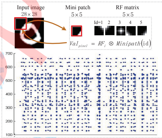
Figure 3 The local feature converting method.
