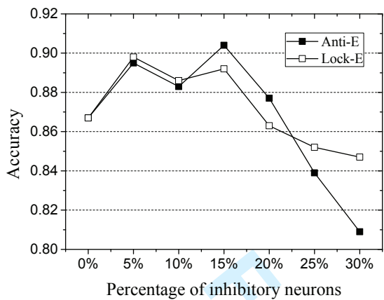
Figure 4 The accuracies of different proportions and types of inhibitory neurons (initial synaptic connection is 50%. All the results are based on the integrated rules of R1, R2, R3, R4, R5b and R6b).
