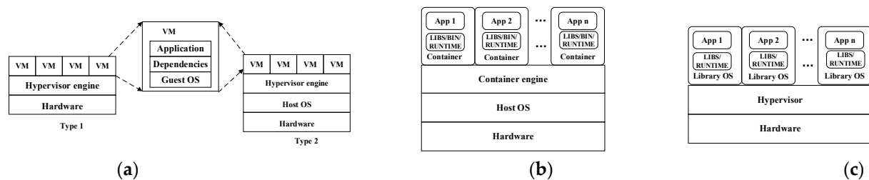
Figure 1. Virtualization Architectures: (a) Virtual machines; (b) Container; and (c) Unikernel.
