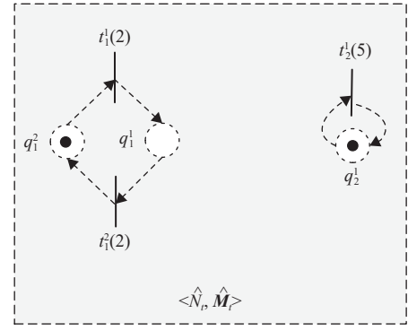
Fig. 3. The equivalent subsystem \langle \hat{N}_t, \hat{M}_t \rangle of transitions.
