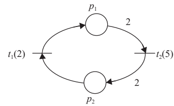
Fig. 2. A TWMG N considered in Examples 1, 2 and 3.
