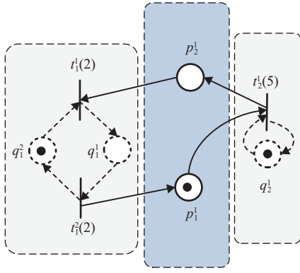
Fig. 5. The equivalent TMG system of the TWMG N depicted in Fig. 2 with M = [2, 0]^T .
