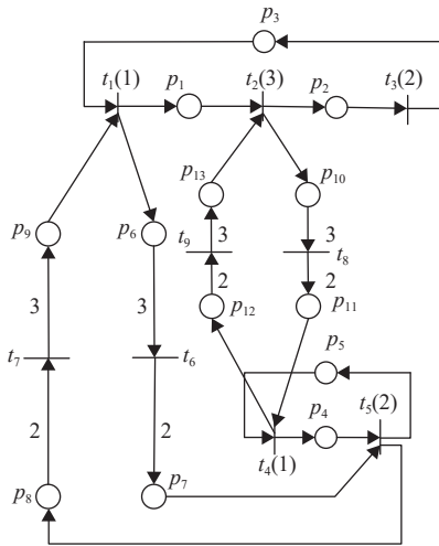
Fig. 6. The TWMG model of a flexible manufacturing system.
