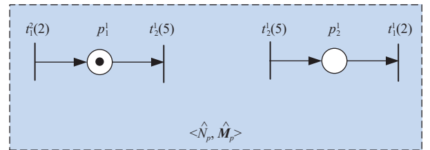
Fig. 4. The equivalent subsystem \langle \hat{N}_p, \hat{M}_p \rangle of places.
