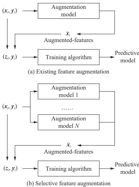
Fig. 2 An intuitive comparison of the training phase between existing feature augmentation techniques and the proposed one in this paper. Here, \mathbf{z}_i is the concatenation of \mathbf{x}_i and \tilde{\mathbf{x}}_i . Specifically, existing feature augmentation techniques focus on designing a better augmentation model to generate more informative augmented features, while this paper focuses on designing a novel training algorithm that aims at synergizing multiple kinds of augmented features.
