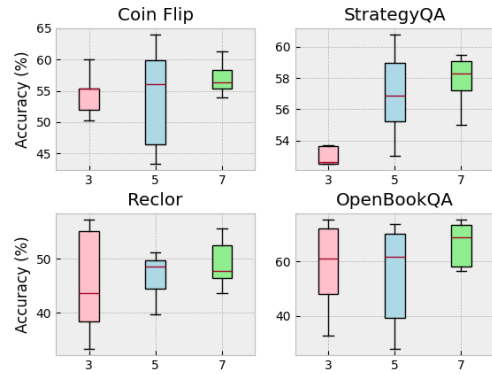
Figure 7: Ablation study on LoRA-Experts. As shown in the results, as the amount of experts reduces (from right to left), reasoning accuracy (%) on four unseen tasks noticeably becomes unstable.
